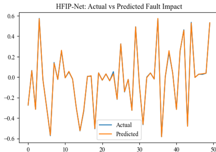
Figure 8: Prediction Fault Impact Comparison Chart
