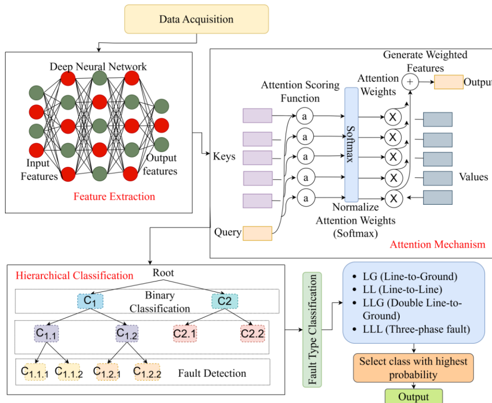
Figure 3: AHA-FCNet Workflow
