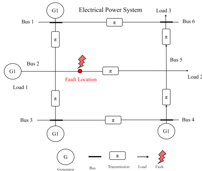
Figure 2: Electrical Power System
