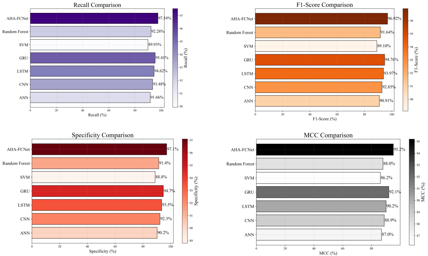
Figure 7: Performances Comparison Chart for AHA-FCNet
