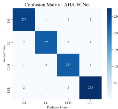
Figure 5: Confusion Matrix for AHA-FCNet
