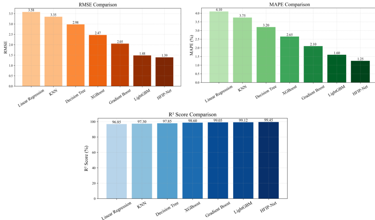
Figure 9: Performances Comparison Chart for HFIP-Net
