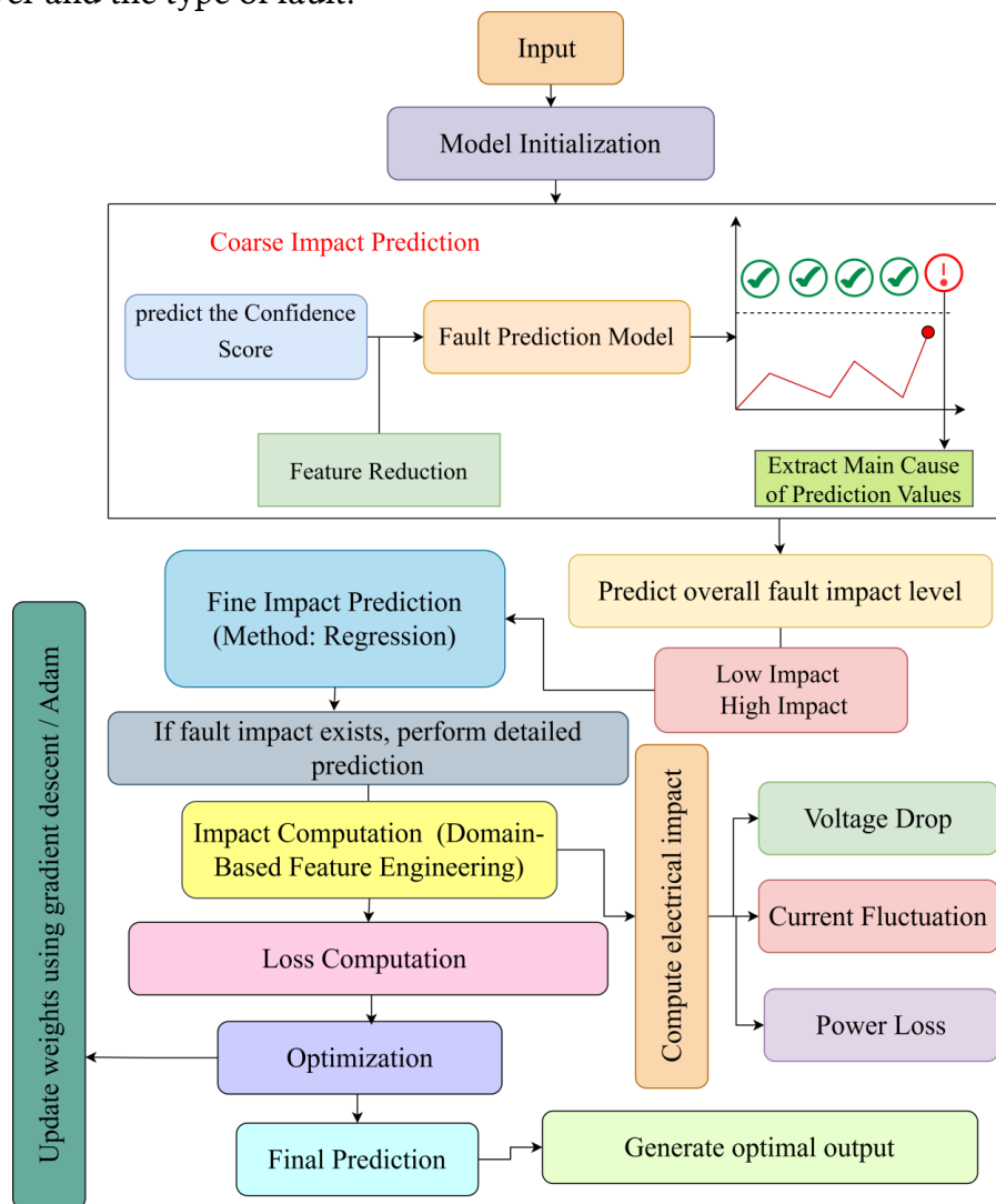
Figure 4: HFIP-Net Workflow
