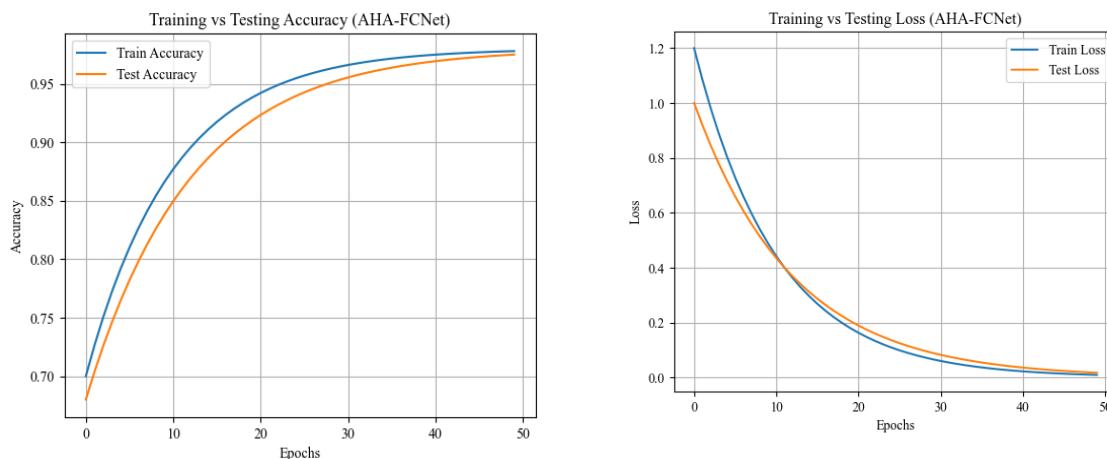
Figure 6: Training and Testing Accuracy and Loss Chart
